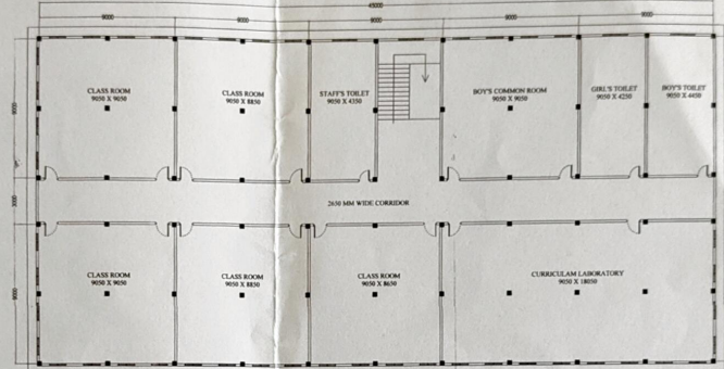
PLAN- FIRST FLOOR SCALE 1:100
