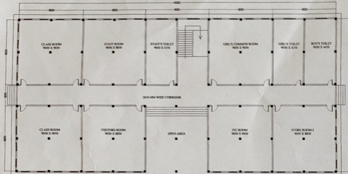
PLAN- GROUND FLOOR SCALE 1:100
