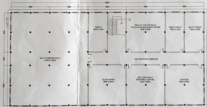
PLAN- SECOND FLOOR SCALE 1:100
