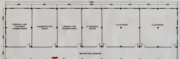
PLAN- EXISTING BUILDING SCALE 1:100
