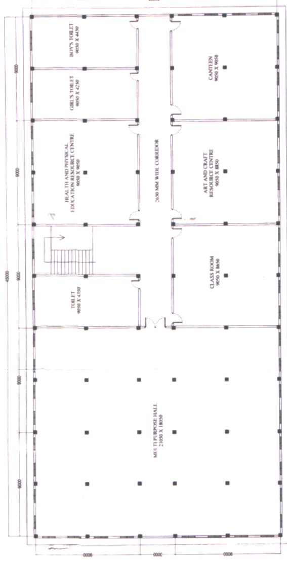
PLAN- SECOND FLOOR SCALE 1:100
